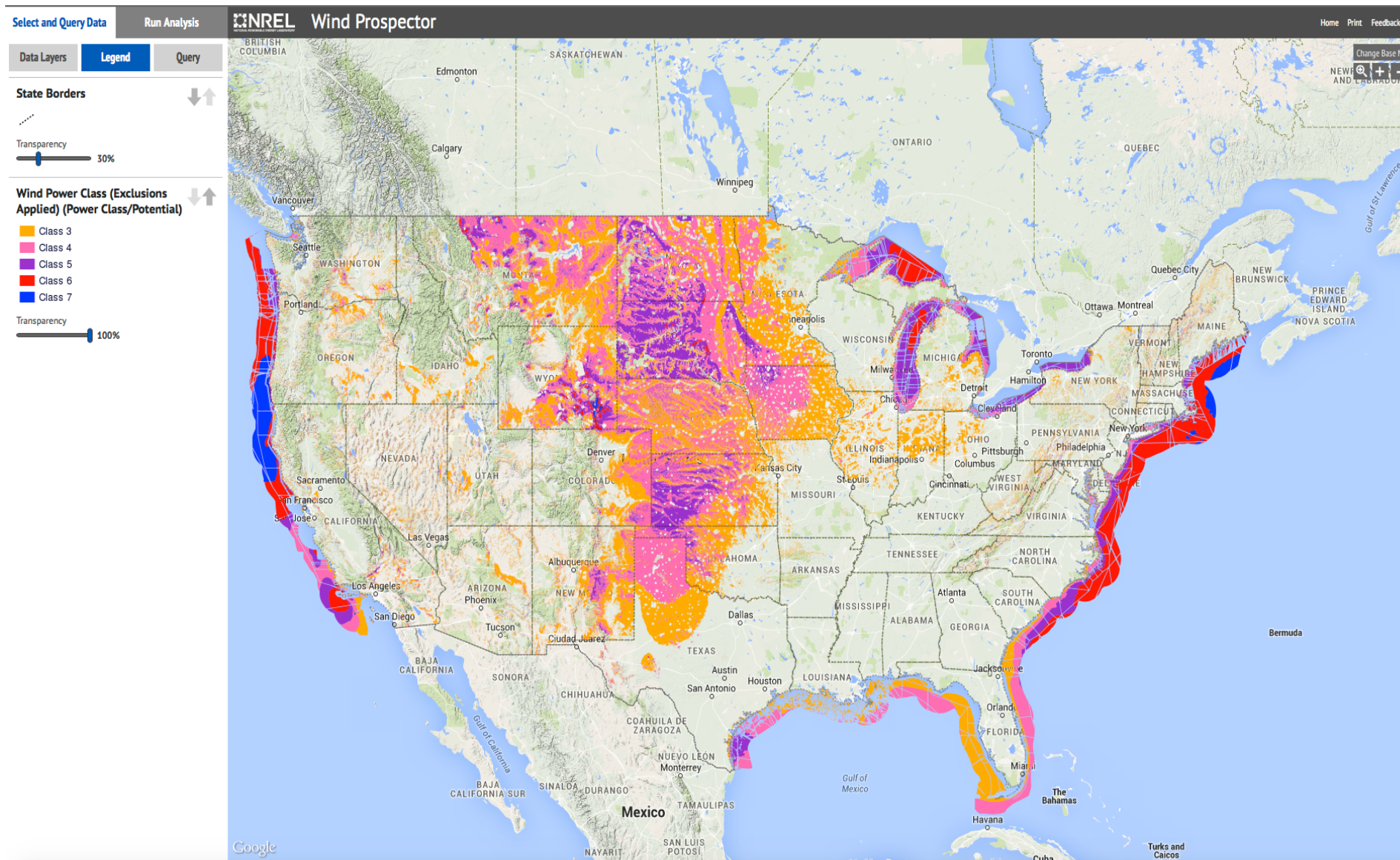
Figure S4. Wind power classes in the, U.S. ( https://mapsbeta.nrel.gov/wind-prospector/ ).
