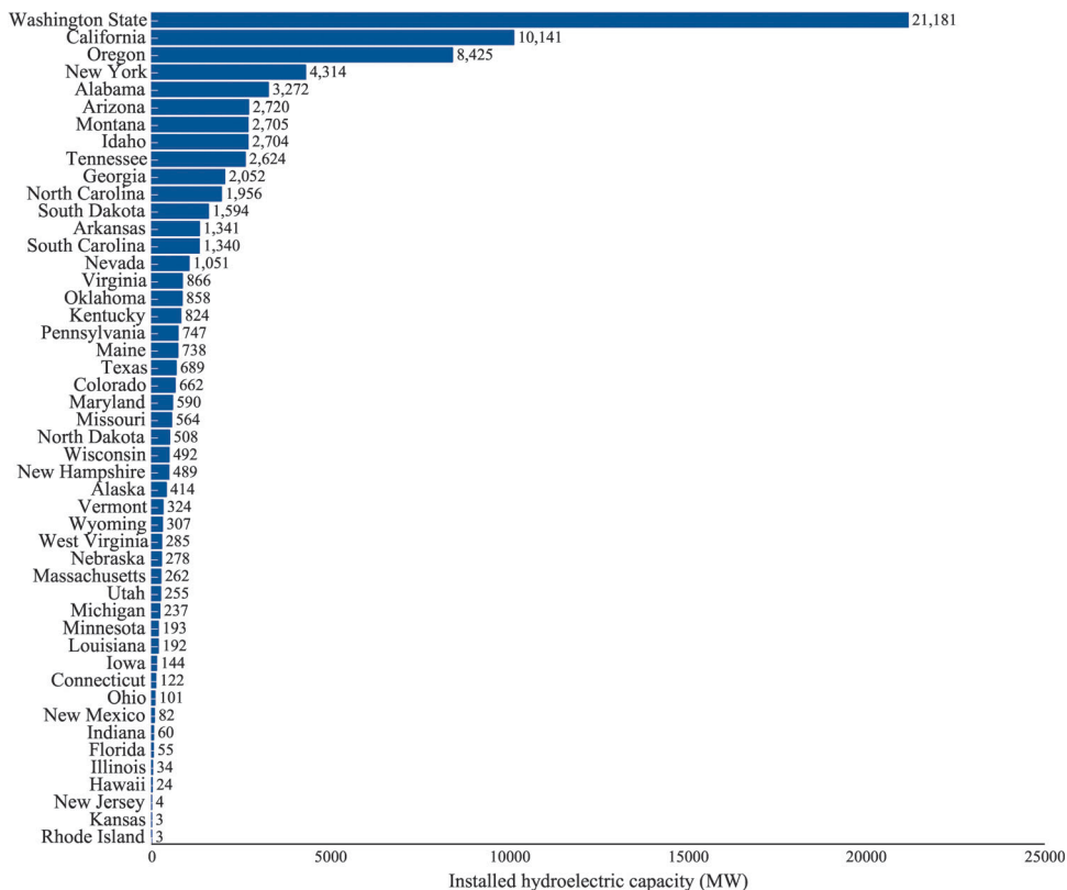
Fig. 4 Installed conventional hydroelectric by U.S. state in 2010. 19
