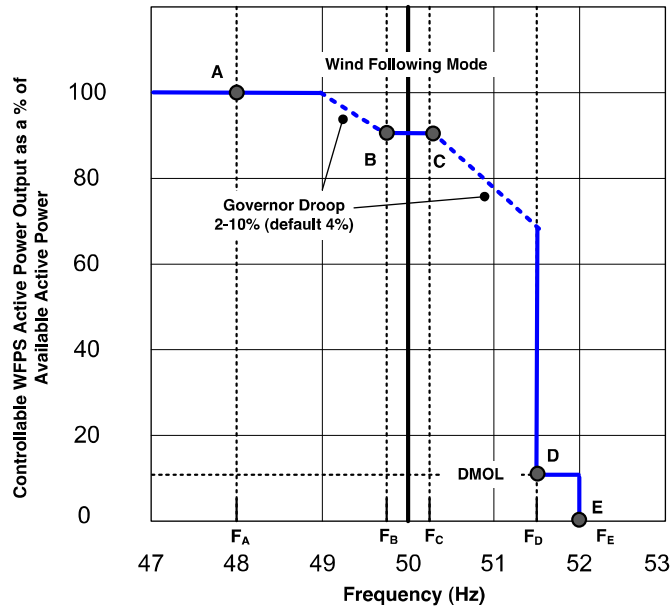
Figure 3 Power-frequency response requirement in Irish Grid Code (EirGrid Code Version 5.0). Outside a frequency deadband (FB-FC) the code requires wind generators to contribute more of the available generation as frequency drops, and to curtail production as frequency increases. Wind is effectively required to provide frequency support service.
