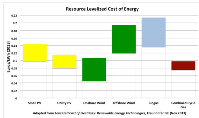
Figure 1 Cost of renewable resources becoming competitive with conventional power plants
